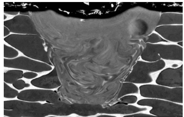
BSE SEM image of a single track melt of Al 0.5 Ce at%
