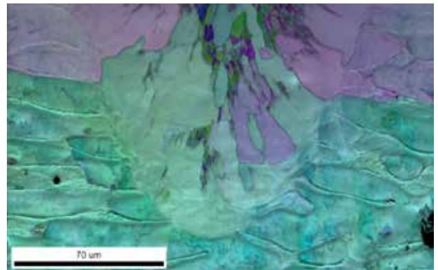
EBSD orientation map of a single track melt of Al 0.5 Co at%
